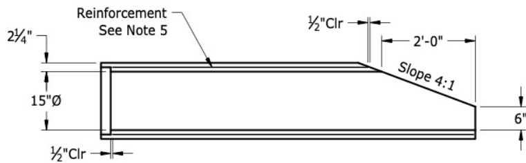
Section View
